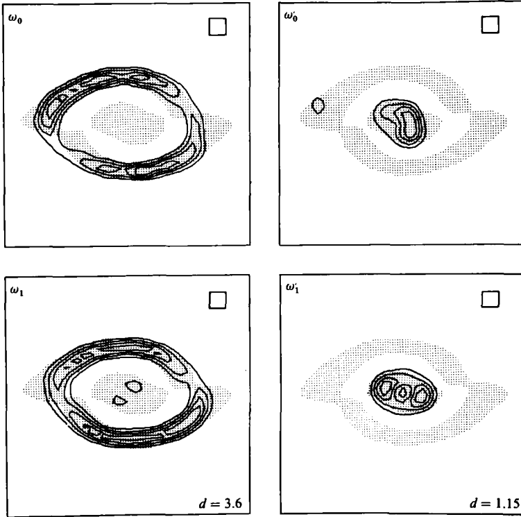
FIGURE 4. Vertical heat-flux correlations \bar{\theta}'u_z'' for several longitudinal ( b = 0 ) unstable modes of the Re = 500 KH wave at the key time (5). The superadiabatic regions of the nonlinear wave (shaded area) have been superimposed on each frame. It can be seen that the \omega_0 and \omega_1 modes are associated with convective activity (positive heat flux) in the primary (ring-shaped) SAR, while the \omega'_0 and \omega'_1 modes are associated with convective activity in the secondary (oval-shaped) SAR. Note that the spanwise wavenumber d was chosen to be near that of the fastest-growing mode for each branch (i.e. d = 3.6 for the \omega_0 and \omega_1 branches and d = 1.15 for the \omega'_0 and \omega'_1 branches). The box in the upper right corner, which has dimensions of L/(N-1) by H/N , shows the nodal spacing of the highest-order Galerkin functions \exp(i\lambda_{\max} \alpha x) and \sin(\nu_{\max} \pi z/H) .
