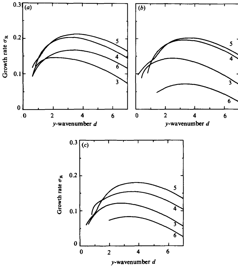
FIGURE 10. Growth rate \sigma_R of the \omega_0 (a), \omega_1 (b) and \omega_2 (c) longitudinal modes as a function of the spanwise wavenumber d for the Re = 500 KH wave at the key times (3), ..., (6) in its energy cycle. (Curves are labelled according to the key time.)
