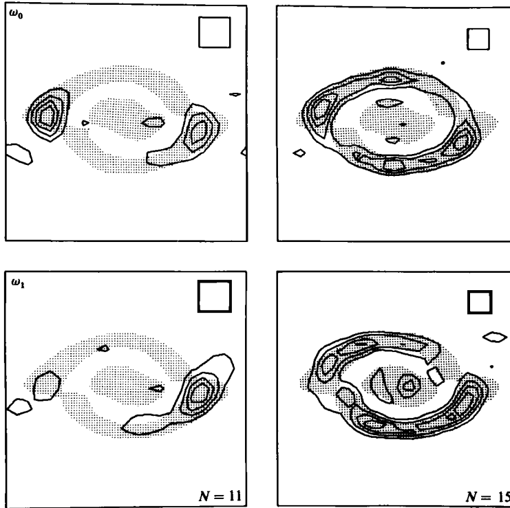
FIGURE 7. Convergence of the vertical heat-flux correlations (\overline{\theta' u_z'}) for the unstable longitudinal \omega_0 and \omega_1 modes of the Re = 500 KH wave at the key time (5). The results shown here at the truncation levels N = 11 and 15 for a spanwise wavenumber d = 3.6 should be compared with those for N = 19 shown in figure 4. The box in the upper-right corner of each frame shows the nodal spacing of the highest-order Galerkin basis functions corresponding to \lambda_{\max} = \frac{1}{2}(N-1) and \nu_{\max} = N .
