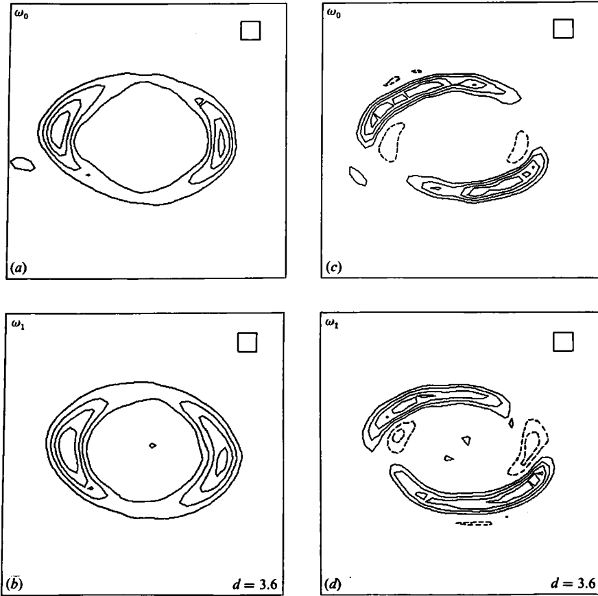
FIGURE 5. (a), (b) Reynolds stress (-\overline{u'_x u'_z}) and (c), (d) (\overline{u'_z})^2 - (\overline{u'_x})^2 correlations for the \omega_0 and \omega_1 modes displayed in figure 4. Note that these correlations are confined to the superadiabatic region.
