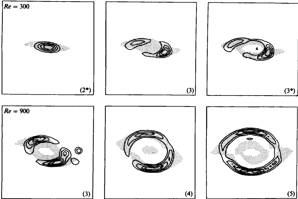
FIGURE 14. Evolution of the vertical heat-flux correlations (\overline{\theta' u_z'}) for the longitudinal \omega_0 modes of the Re = 300 and 900 KH waves. The spanwise wavenumber d = 1.7 for Re = 300 , while d = 4.7 for Re = 900 . The key times are indicated in the lower-right corner of each frame. Note the correlation of the convective activity (positive heat flux) with the primary portion of the (shaded) SAR.
