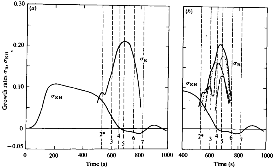
FIGURE 8. Time dependence of the non-dimensional growth rates \sigma_R of the non-oscillatory (a) and oscillatory (b) longitudinal modes of the Re = 500 KH wave (with spanwise wavenumber d = 3.6 and truncation level N = 19 ). Note that the time axis is in units of seconds. The instantaneous growth rate \sigma_{KH} of the KH wave provides an indication of the magnitude of temporal variations in the nonlinear wave. The vertical dashed lines indicate the key times in the energy cycle of the KH wave. Key for the oscillatory modes: —, \omega_1 ; ····, \omega_2 ; ----, \omega_3 ; -·-, \omega_4 .
